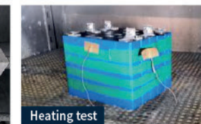
Heating test
